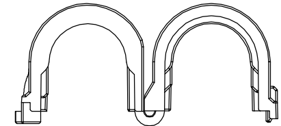
OPEN VIEW OF LOCKOUT DEVICE
